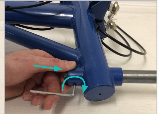
FIGURE 3.2.3 With the shaft inserted all the way forward, secure the shaft by tightening the set screw with the 3 mm hex wrench.
