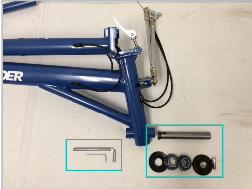
FIGURE 3.2.1 Lay the frame on its left side. Retrieve the front beam shaft assembly, take the cap, tapered bearings and back plate off the shaft, and get the 8 and 3 mm hex wrenches.
