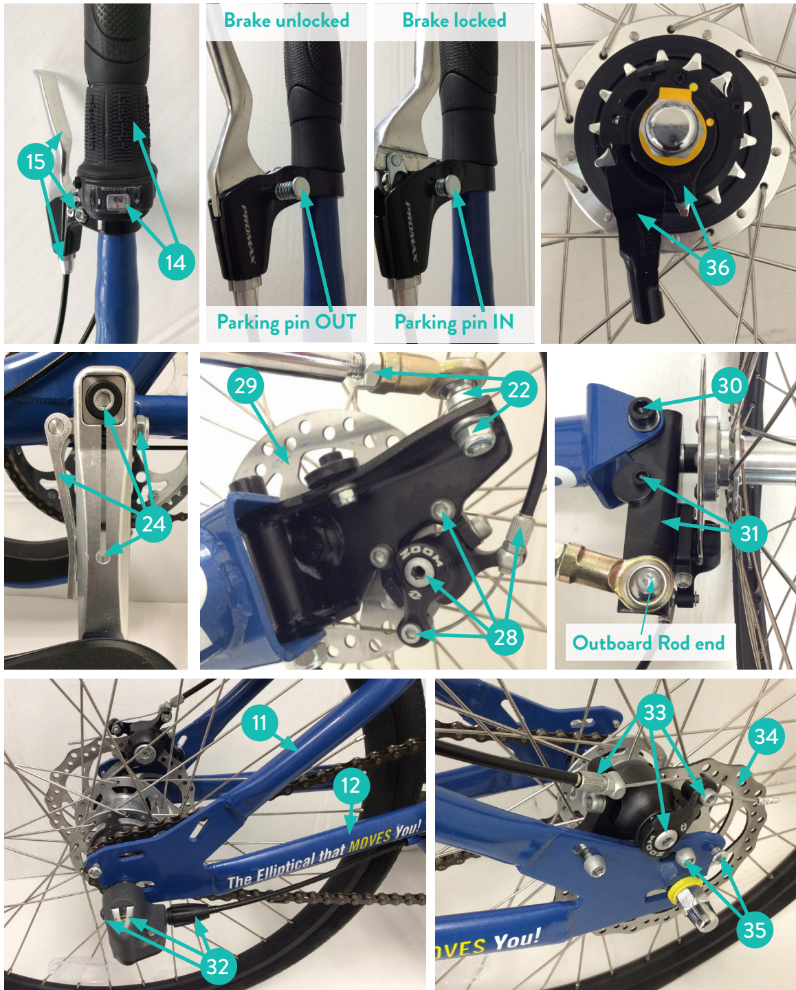
Figure 2.2 StreetStrider 3i and 7i Parts. Refer to Table 2.1 for part numbers and descriptions.
