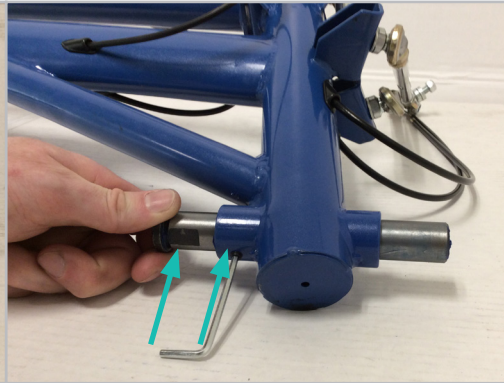
FIGURE 3.2.2 Loosen the set screw under the front beam shaft tube with a 3 mm hex wrench. Slide the shaft into the tube so that the flat section on the rear end of the shaft fits just above the 3 mm screw set.
