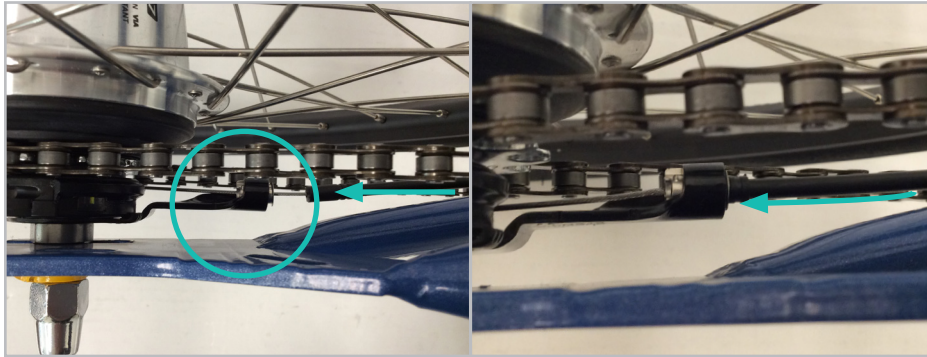
FIGURE 3.6.5 While holding the wrench at the 6 o'clock position, pull the shifter cable housing forward until the cable can be slid into the slot of the arm of the cassette pulley, push the black plastic ferrule on the end of the cable housing into the socket, then return the wrench to the 9 o'clock position making sure the cable lies in the groove under the cassette pulley.
