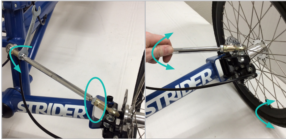
FIGURE 3.7.2 If distances are not equal, use the 14 mm open end wrench to loosen the jam nuts that are tightened against the base of each rod end. On each steering linkage, one rod end has right hand threads and the other has left hand threads, so make sure to turn the jam nuts in the correct direction to loosen. Rotate the linkage rod one way or the other- note how the tire angle changes - until the distance between the tire center ribs in the front is equal to that in the rear and the wheels are parallel while making sure that the cross bar stays horizontal.
