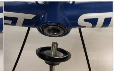
FIGURE 3.2.7 Insert the bearing and other bearing onto the shaft with the taper facing rearward. Put the cap over the front of the beam shaft, insert the 10 mm screw, and tighten with the 8 mm hex wrench.
