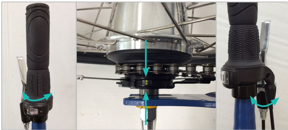
FIGURE 3.6.6 To check gear alignment, twist the shifter to gear 4 and make sure the 2 yellow lines in the cassette pulley window are in line. If the lines are offset, use the barrel adjuster nut at the shifter to move the lines into the correct position.
