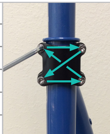
FIGURE 3.4.15 With the 4 mm hex wrench, carefully tighten the Joint #1 clamp in an X pattern so that all the screws are tightened evenly and the space between the clamp base and cap on the front side of the pole is equal to the space on the rear side.
