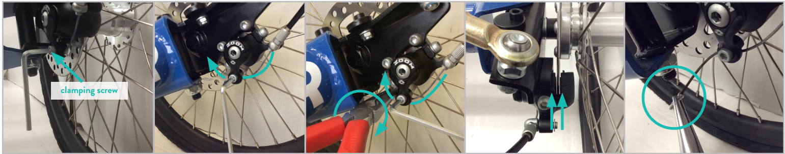
FIGURE 3.5.3 Loosen the clamping screw with the 4 mm hex wrench so there is space to route the brake cable under the nut. Grip the brake cable end with pliers, rotate the pliers to make the cable taut, then tighten the cable clamping screw. Unscrew the inner and outer brake pads so that a sliver of light can be seen between the rotor and pads and so the wheel spins freely. Bend the cable away from rotor and squeeze a cable tip onto the end of each cable. Repeat on the other brake.
