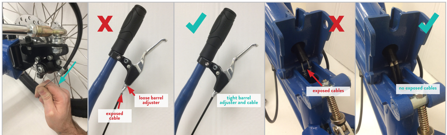
FIGURE 3.5.2 Pull each of the brake cables down at the right and left brake calipers to make sure there is no exposed cable visible at the brake lever or at the cable doubler by inserting the cable housing ferrules into the barrel adjusters and doubler.
