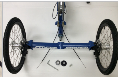
FIGURE 3.2.5 Unfold the front wheels on the front beam and set the front wheel assembly in front of the shaft.
