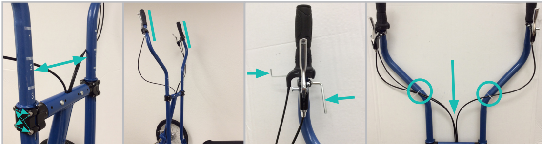
FIGURE 3.18.15 Attach the lower and upper pole on the left side following the procedure used on the right side. Make sure the left and right poles are set to the same height, rotate the poles to approximately shoulder width of the user and also parallel from the side view.
